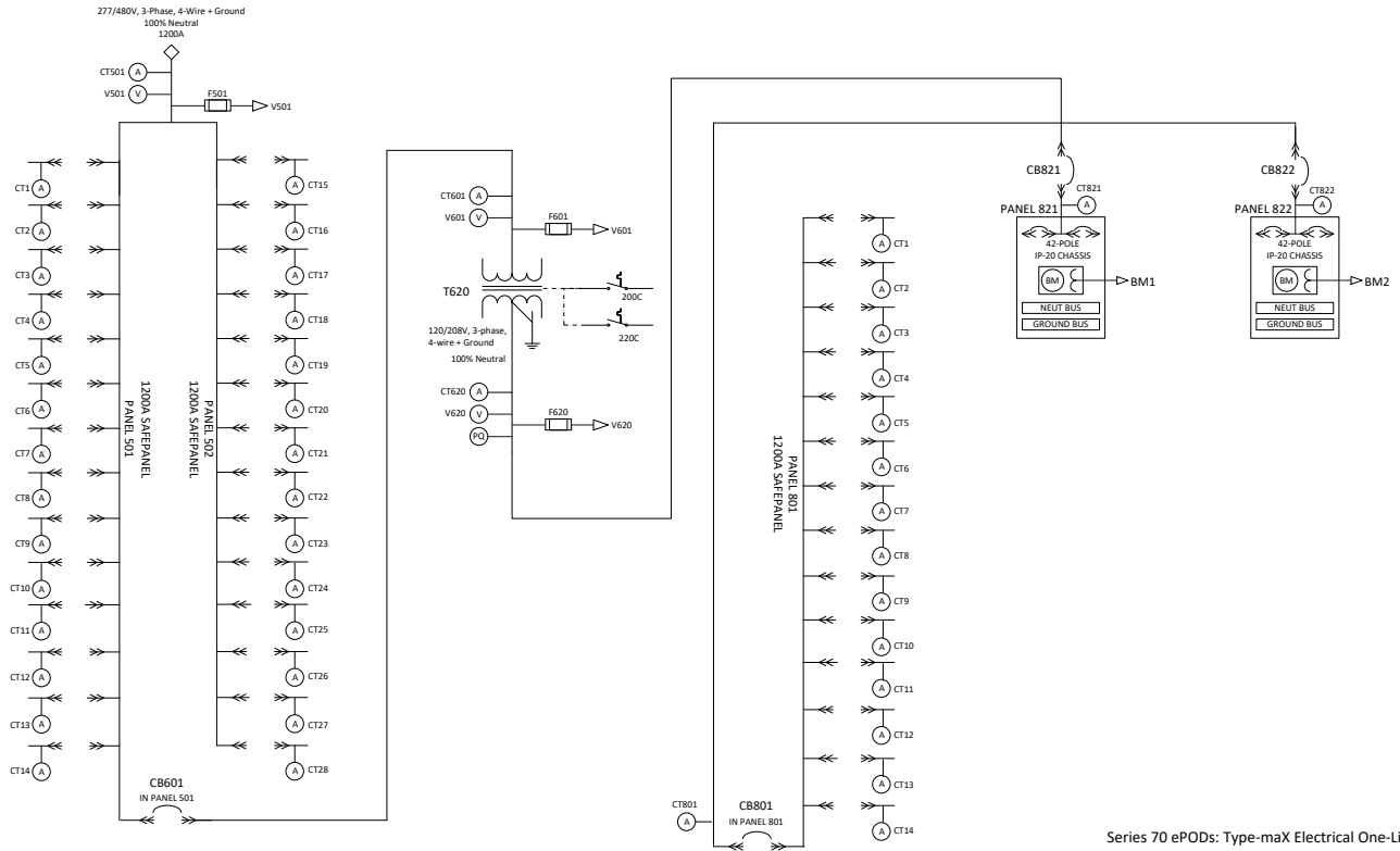
Series 70 ePODs: Type-maX Electrical One-Line Diagram
